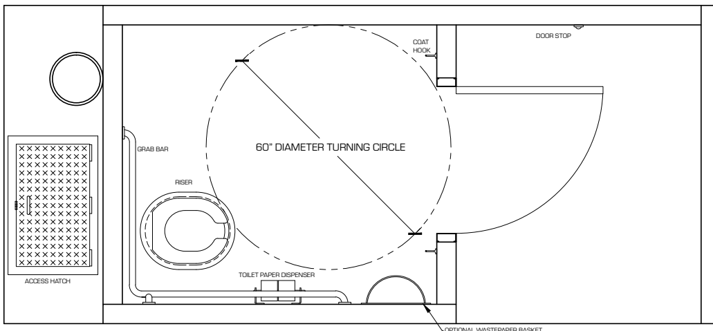
Standard Floor Plan with Options Shown (for reference only)
